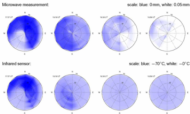
Figure 2. Hemispheric Integrated Liquid Water and Infrared Cloud Temperature distributions above Bern on April 8, 2003 as derived from ASUMUWARA. After [18].
