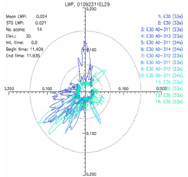
Figure 3. Series of 14 successive azimuth scans at 30 deg elevation with the multi-channel microwave radiometer MICCY having a beam width of less than 1 deg in all channels. Liquid water path was derived using a regression algorithm employing four frequency channels. Venema [Private communication].
