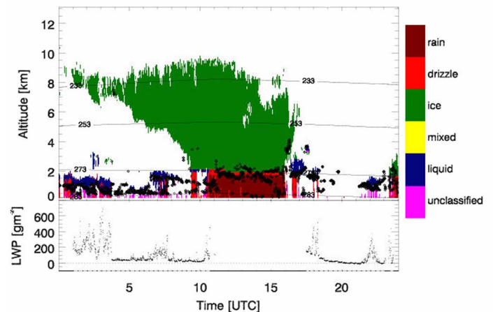
Figure 4. Cloud classification and LWP for May 19, 2003 at Cabauw. Temperature is derived from interpolated radiosondes. The classification is performed for each individual cloud radar range gate. Black dots indicate the cloud base height as observed by lidar ceilometer.
