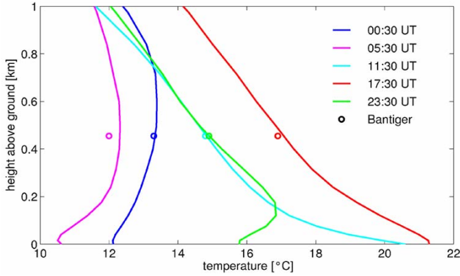
Figure 1. Temperature profiles in the lowest km above ground at 5 different times on September 18, 2002 in Bern measured with ASUMUWARA and comparison with data from a meteo station (circles) located on a nearby TV tower. After [18].
