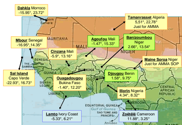
Figure 2. AERONET (yellow), IDAF (blue) and both AERONET/IDAF (green) ground-based stations.
