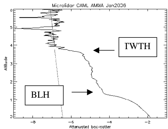
Figure 4 : Example of retrieved attenuated backscattering coefficient (ABC, solid line) in decimal logarithmic scale ( x is 10^x \text{ m}^{-1} \text{ sr}^{-1} ) as a function of altitude (1 mn and 75m resolution). Dotted line is molecular backscattering from the seasonal model used for normalization. The boundary layer height (BLH) and the trade wind layer top height (TWTH) can be obtained from the analysis of the ABC.
